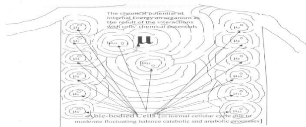
Figure 2. Balance Internal Energy both cells and an organism due to their chemical potentials ( \mu ) promoting operation resonance waves of cellular capacitors.
